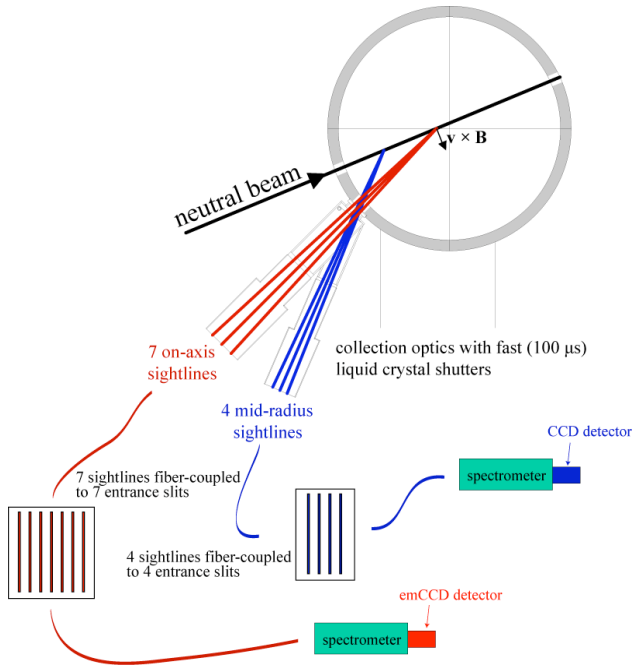
Fig. 1. The MSE diagnostic has an on-axis view and a new mid-radius view. Each view contains multiple sightlines of the diagnostic neutral beam.
