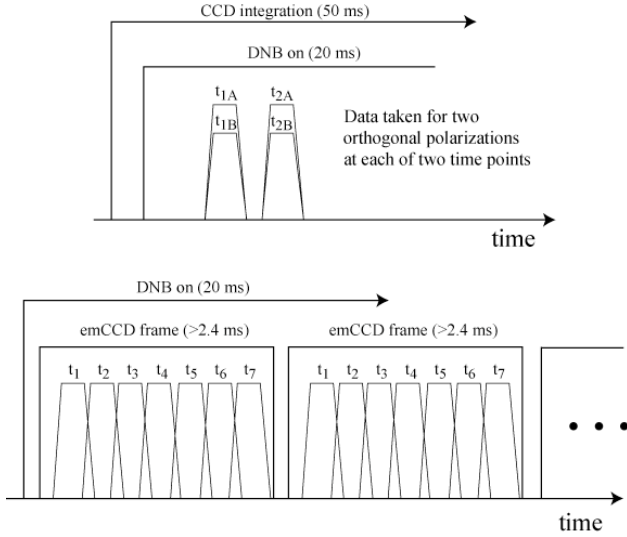
Fig. 3. Timing diagrams illustrating the sequence of events during operation of the MSE diagnostic. The lower diagram represents collection of seven sequential spectra from the on-axis view on a single emCCD frame, a sequence repeated after each frame is read out; multiple such sequences are recorded during each 20 ms DNB pulse. The upper diagram represents collection of two sequential sets of spectra from the mid-radius view on a single CCD frame, not repeated during a DNB pulse because the CCD frame readout is slow.
