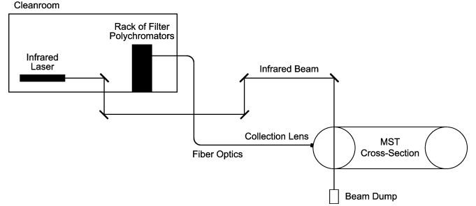
Fig. 4. Layout of the Thomson scattering diagnostic on MST. The laser systems and banks of filter polychromators are in a temperature-controlled room approximately 12 m remote from the MST torus.
