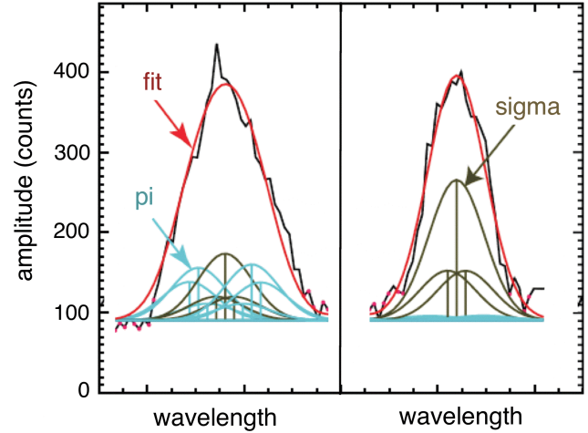
Fig. 2. Sample spectra from the mid-radius view, the two panels containing spectra from two sightlines set up to collect orthogonal polarizations simultaneously. The position and broadening of the \pi and \sigma components are illustrated, along with the fit to the recorded spectra. The derived |\mathbf{B}| = 0.42 \pm 0.07 T and the pitch angle \gamma = 40.3^\circ \pm 9.4^\circ .
